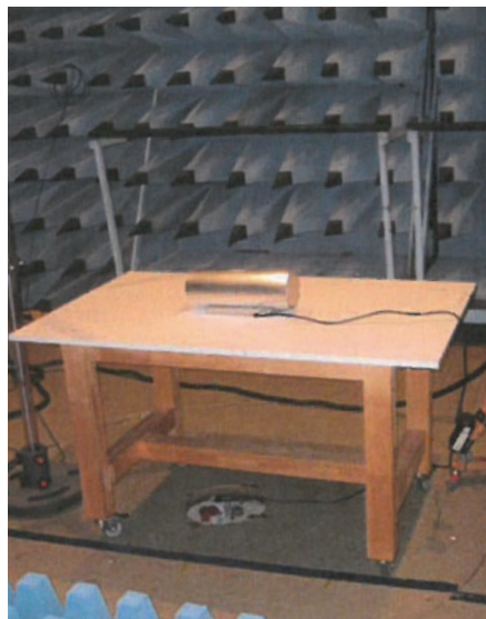
MEASURING voltage fluctuations
